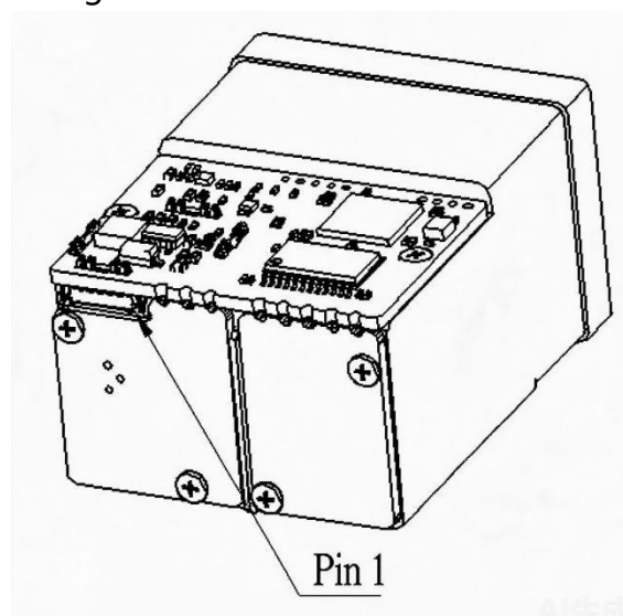
Figure 3: Connector Pin 1 Location
