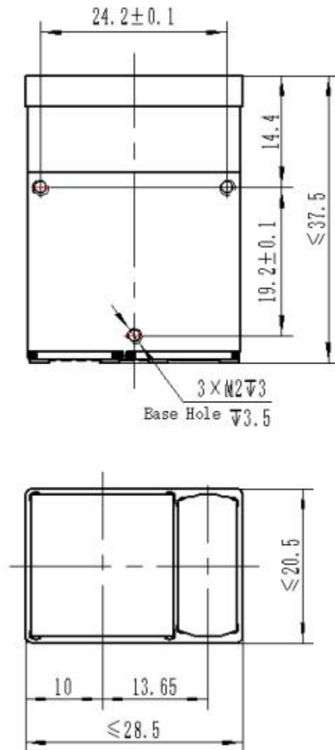
Figure 2: Mechanical and Optical Interface Diagram
